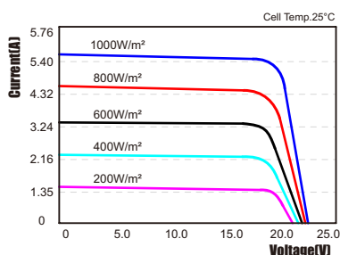
I-V Curves of PV module SY-M90W
