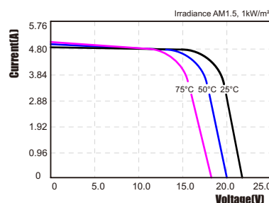
I-V Curves of PV module SY-M90W at various cell temperatures
