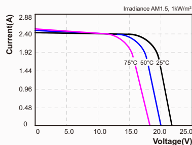
I-V CurvesofPVmoduleSY-M40Watvariouscell temperatures
