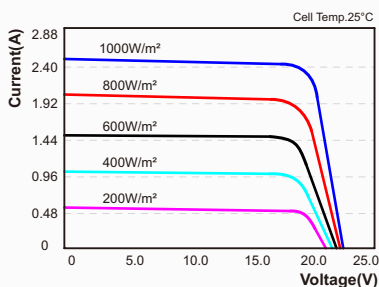
I-V CurvesofPVmoduleSY-M40W
