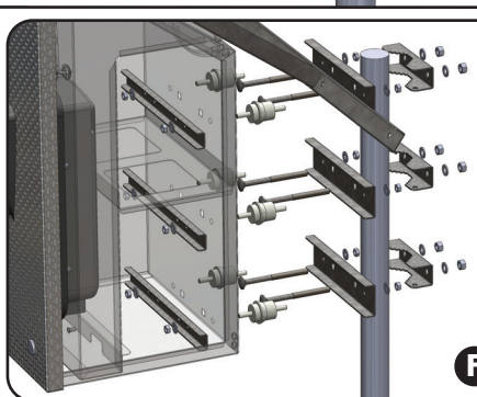
Nuts attached and tightened
