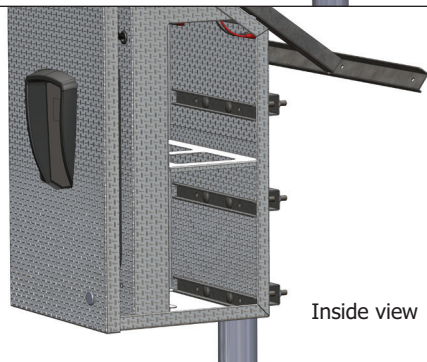
Bolts through from inside
