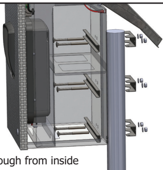
Nuts attached and tightened
