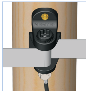
Poly tape tensioned and live (AS-TRS40SS)
