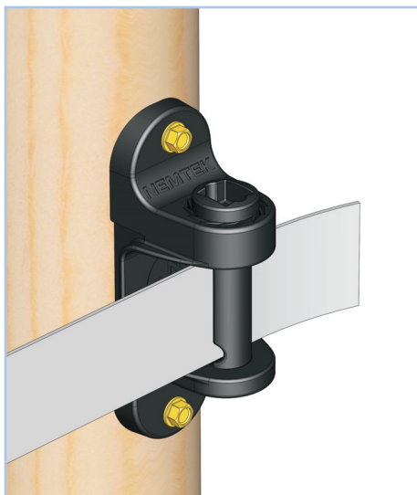
Feeding the 40mm poly tape through the spindle.
