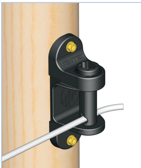
Feeding the 6mm poly braid through the spindle.
